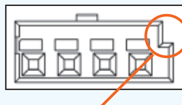
D1-Connector: V-Coding – contact pins Tin-plated
